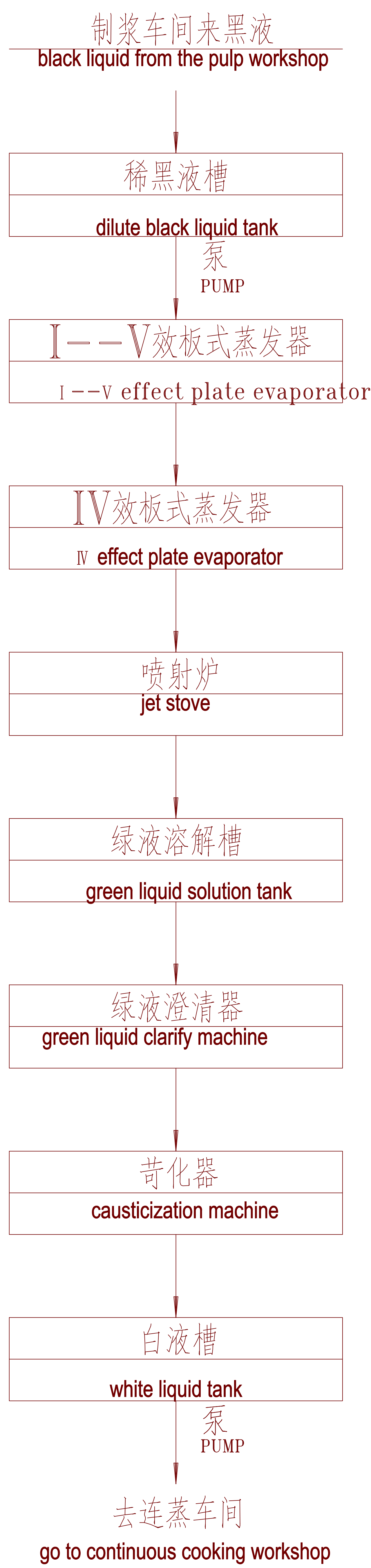
alkali recycling workshop process line diagram
