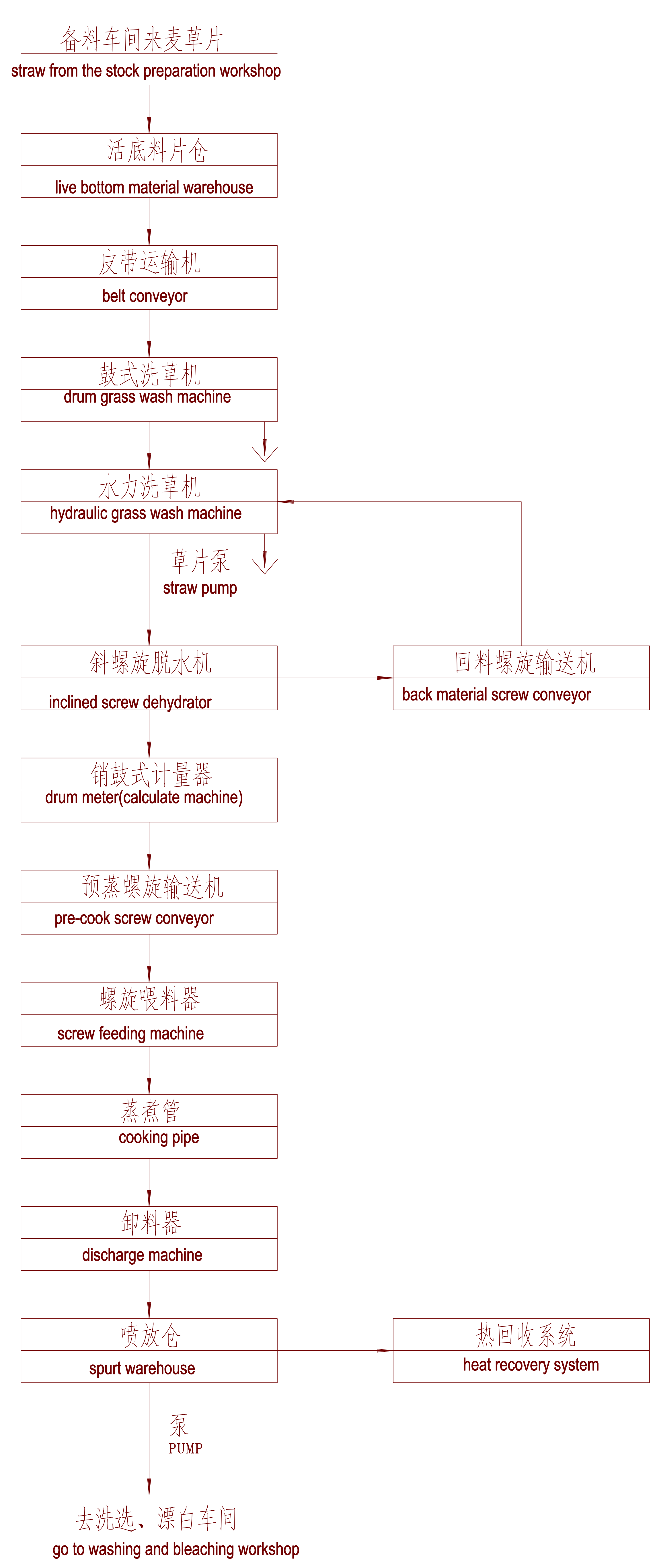
连续蒸煮车间流程简图 continuous cooking workshop process line diagram
