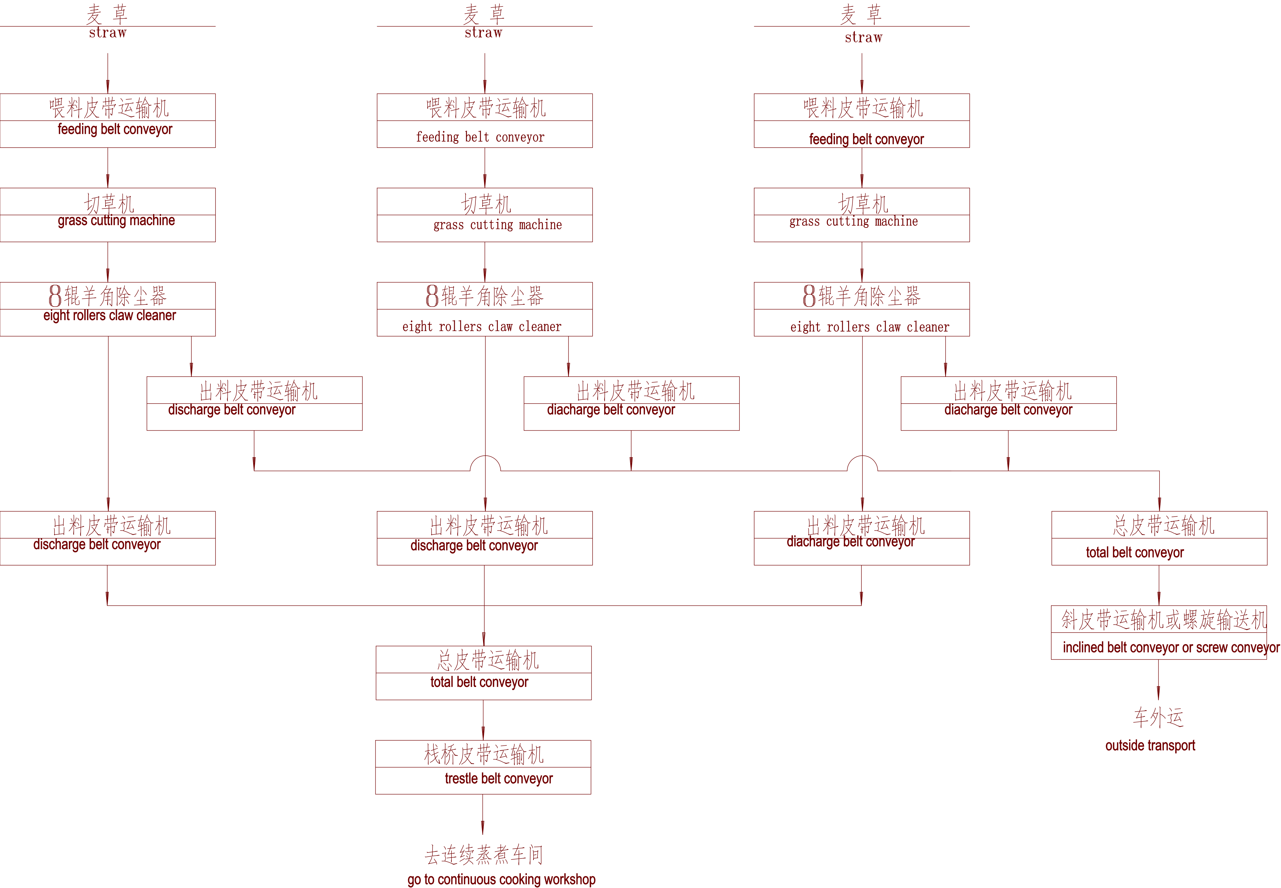
stock preparation workshop process line diagram
